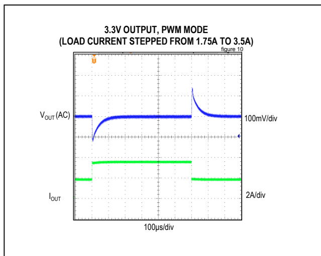
Figure 10. MAX17504 3.3V Output, 1.75A to 3.5A Load Transient
