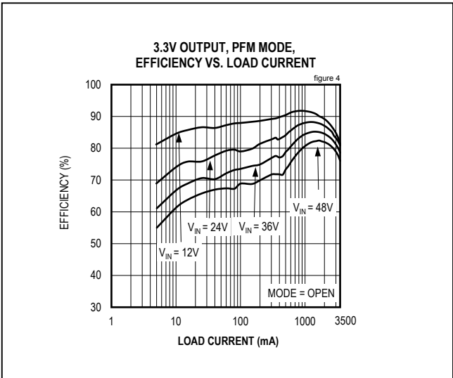
Figure 4. MAX17504 3.3V Output Efficiency (PFM Mode)
