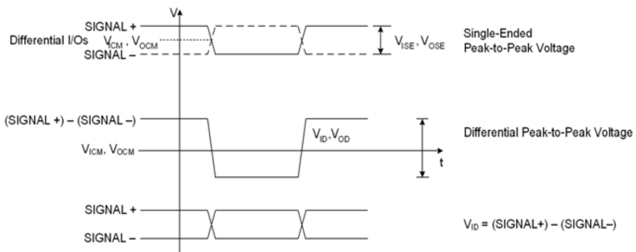
Figure 1. Voltage Characteristics
