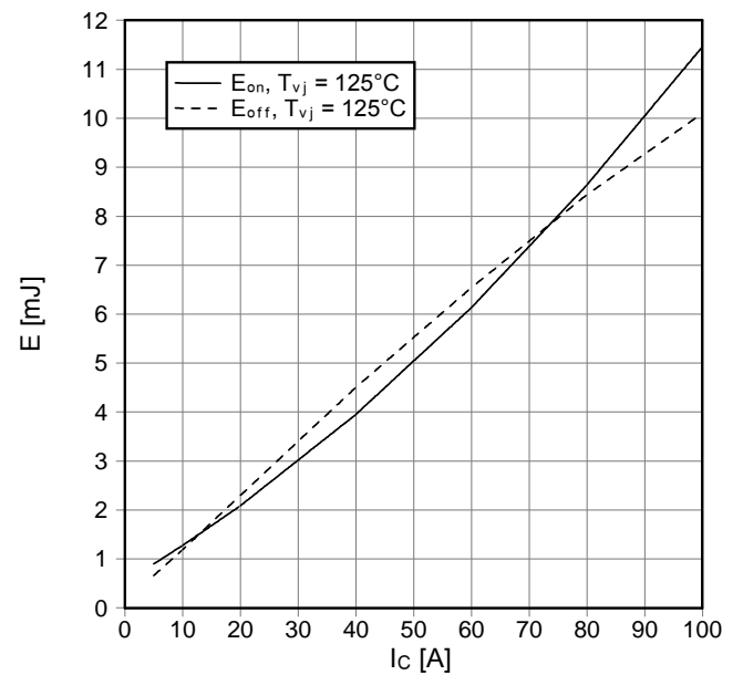
Schaltverluste IGBT-Wechselr. (typisch) switching losses IGBT-inverter (typical) E_{on} = f(I_C) , E_{off} = f(I_C) V_{GE} = \pm 15\text{ V} , R_{Gon} = 18\ \Omega , R_{Goff} = 18\ \Omega , V_{CE} = 600\text{ V}
