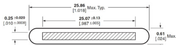
Single Conductor
