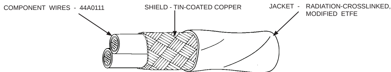
CABLE CONSTRUCTION DETAILS
