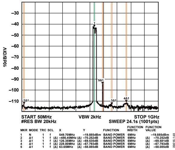
Figure 49. Mid Band Wideband ACLR
