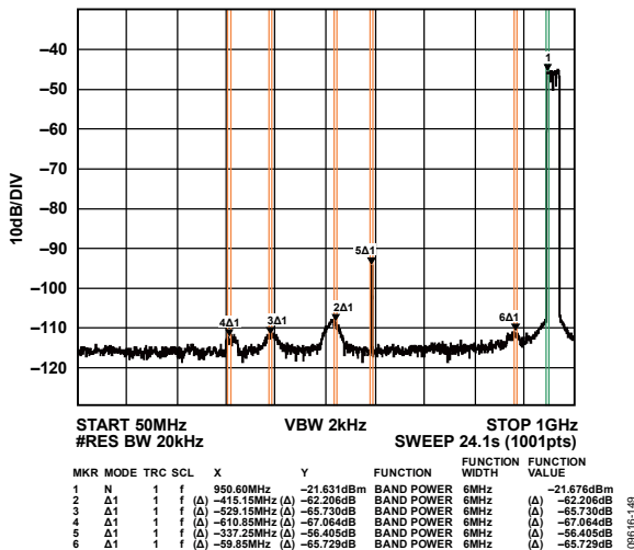
Figure 50. High Band Wideband ACLR
