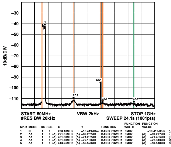
Figure 48. Low Band Wideband ACLR
