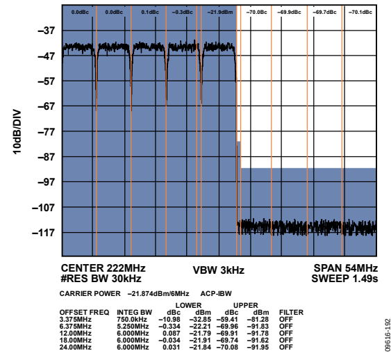
Figure 131. Low Band Narrow-Band ACLR (Worse Side)
