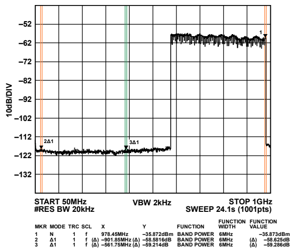
Figure 147. 64-Carrier High Band Wideband ACLR
