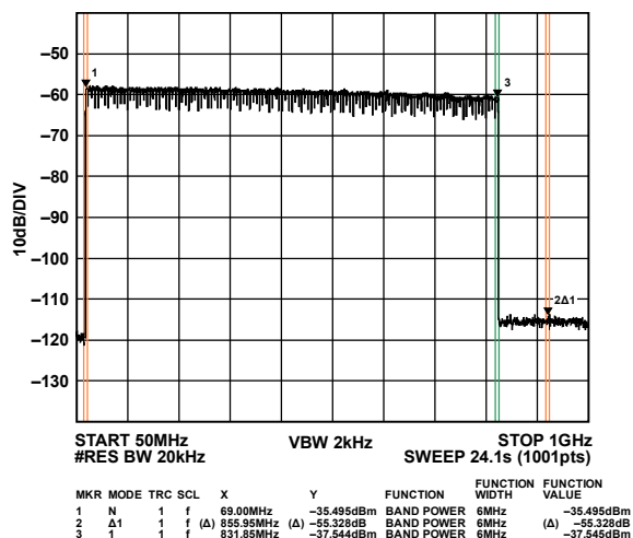
Figure 148. 128-Carrier Wideband ACLR
