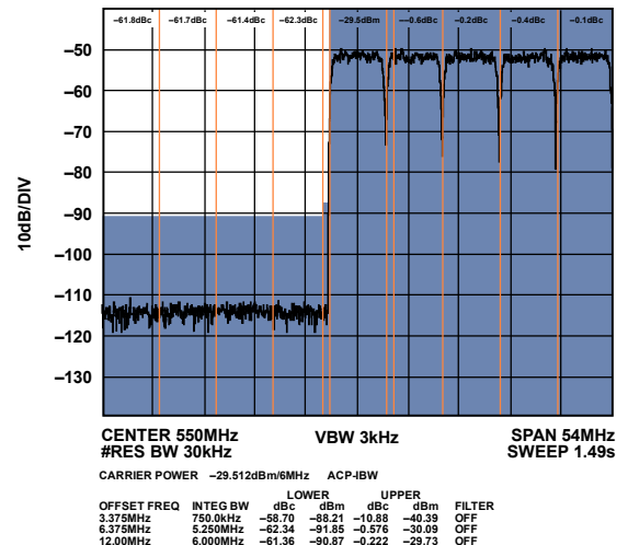
Figure 70. Mid Band Narrow-Band ACLR (Worse Side)
