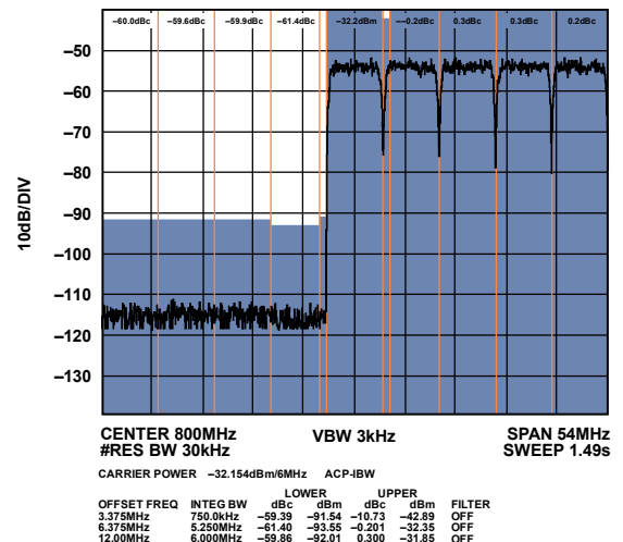
Figure 71. High Band Narrow-Band ACLR
