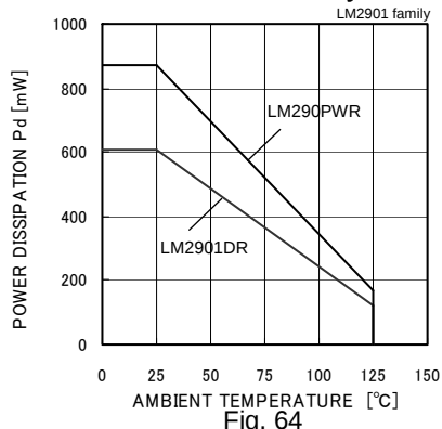
Fig. 64 Derating Curve
