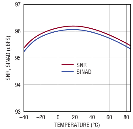
SNR, SINAD vs Temperature, f_{\text{IN}} = 2\text{kHz} , -1dBFS
