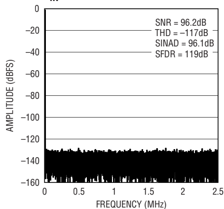
32k Point FFT f_{\text{SAMPL}} = 5\text{Mps} , f_{\text{IN}} = 2\text{kHz}
