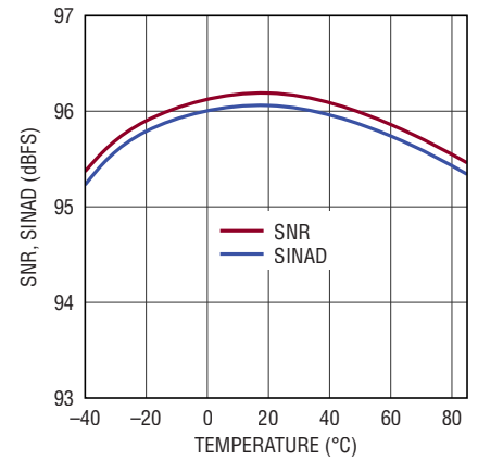
SNR, SINAD vs Temperature, f_{\text{IN}} = 2\text{kHz} , -1\text{dBFS}
