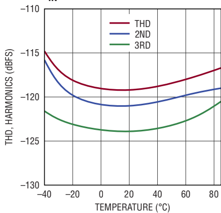
THD, Harmonics vs Temperature, f_{\text{IN}} = 2\text{kHz} , -1\text{dBFS}
