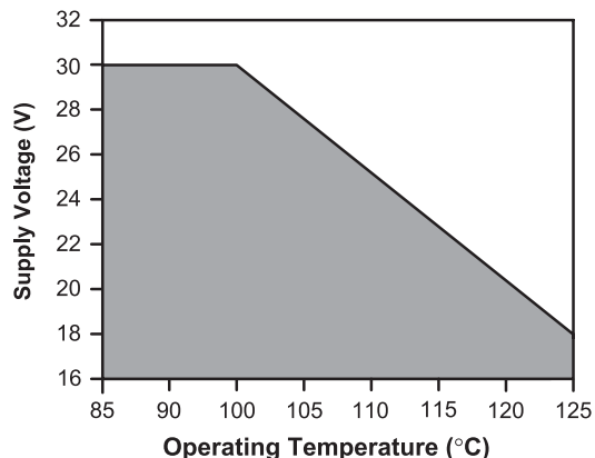
Figure 2. Regulated Output Supply Voltage
