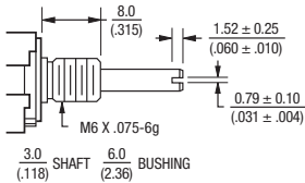
S Style Bushing
