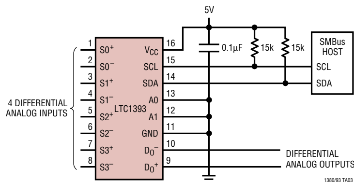
Simplified LTC1393 Application
