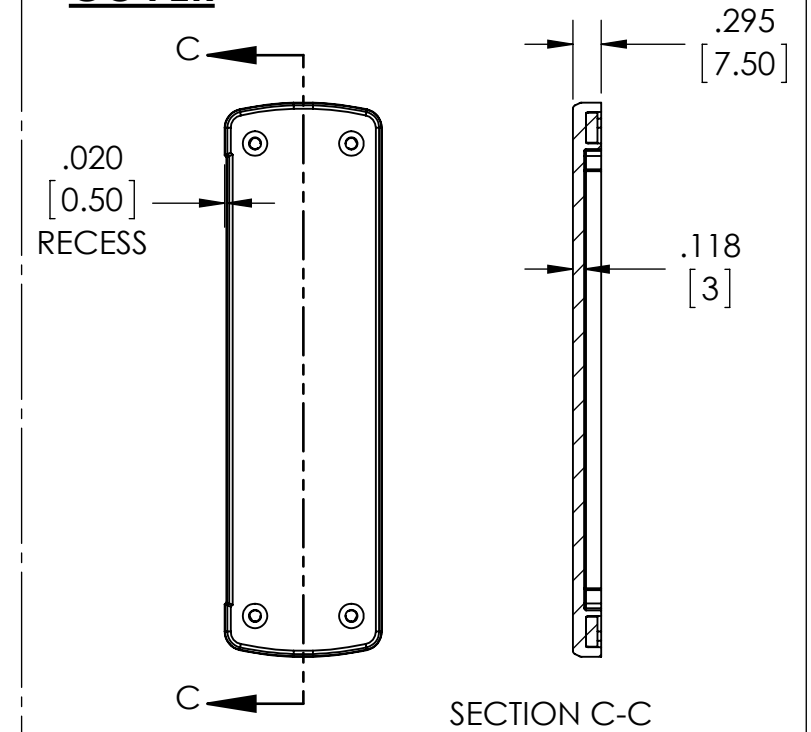
PLASTIC COVER
