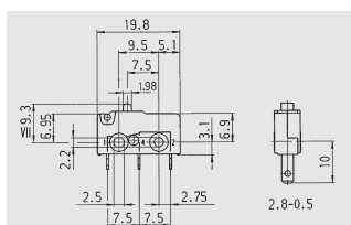
quick-connect
