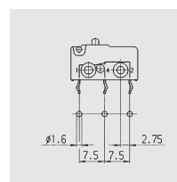
bent PCB terminal
