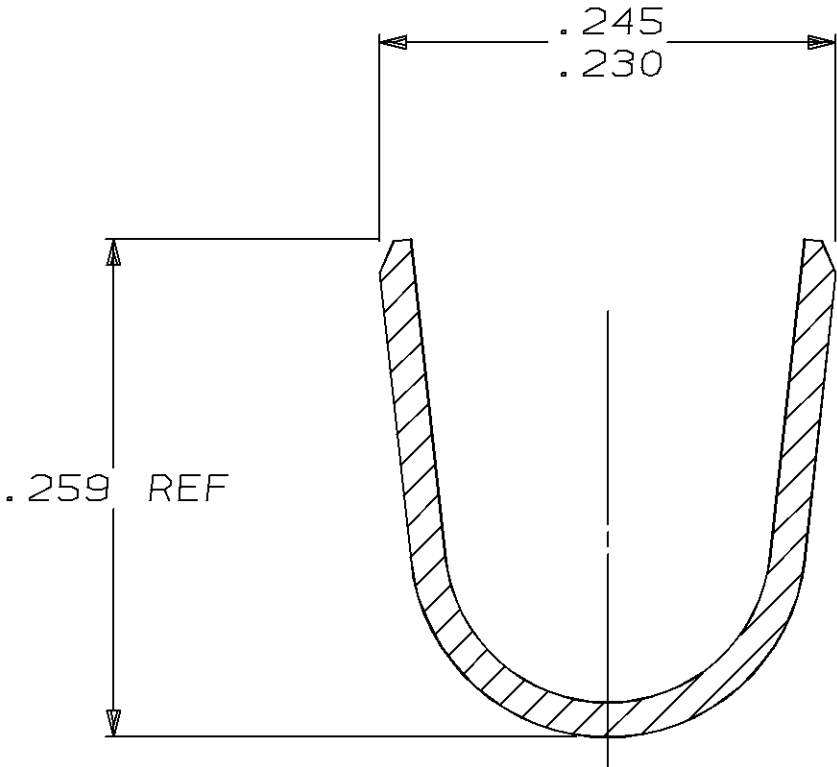
SECTION B-B SCALE 10:1
