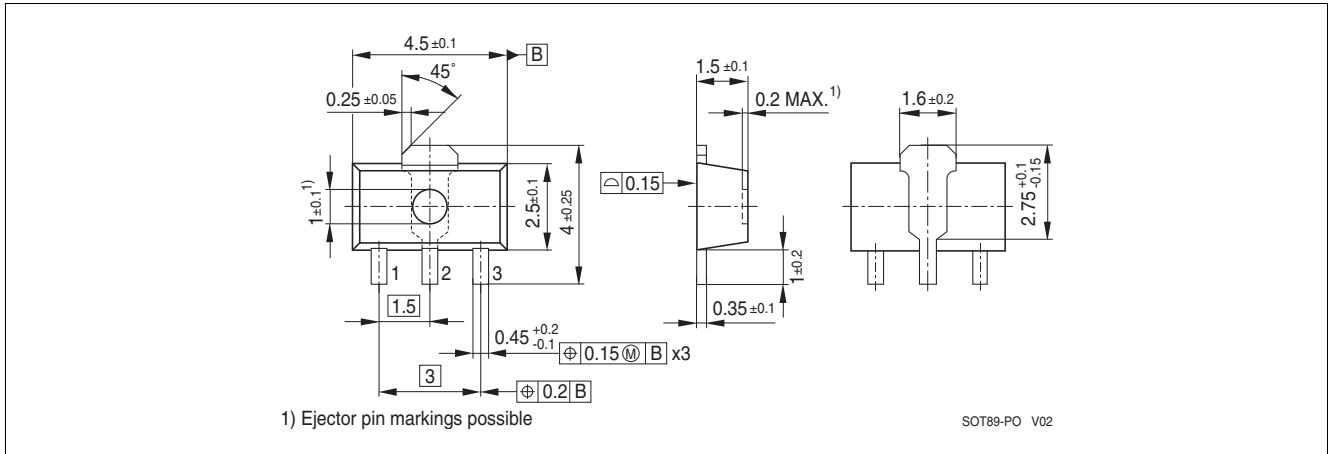
Figure 1 Package Outline
