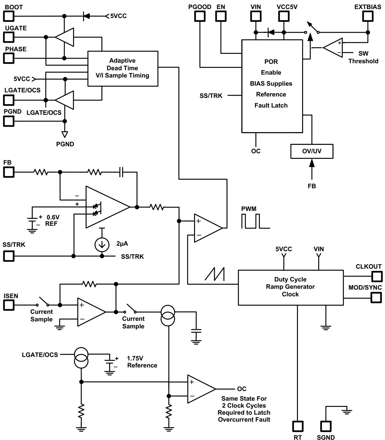
Figure 3. Block Diagram
