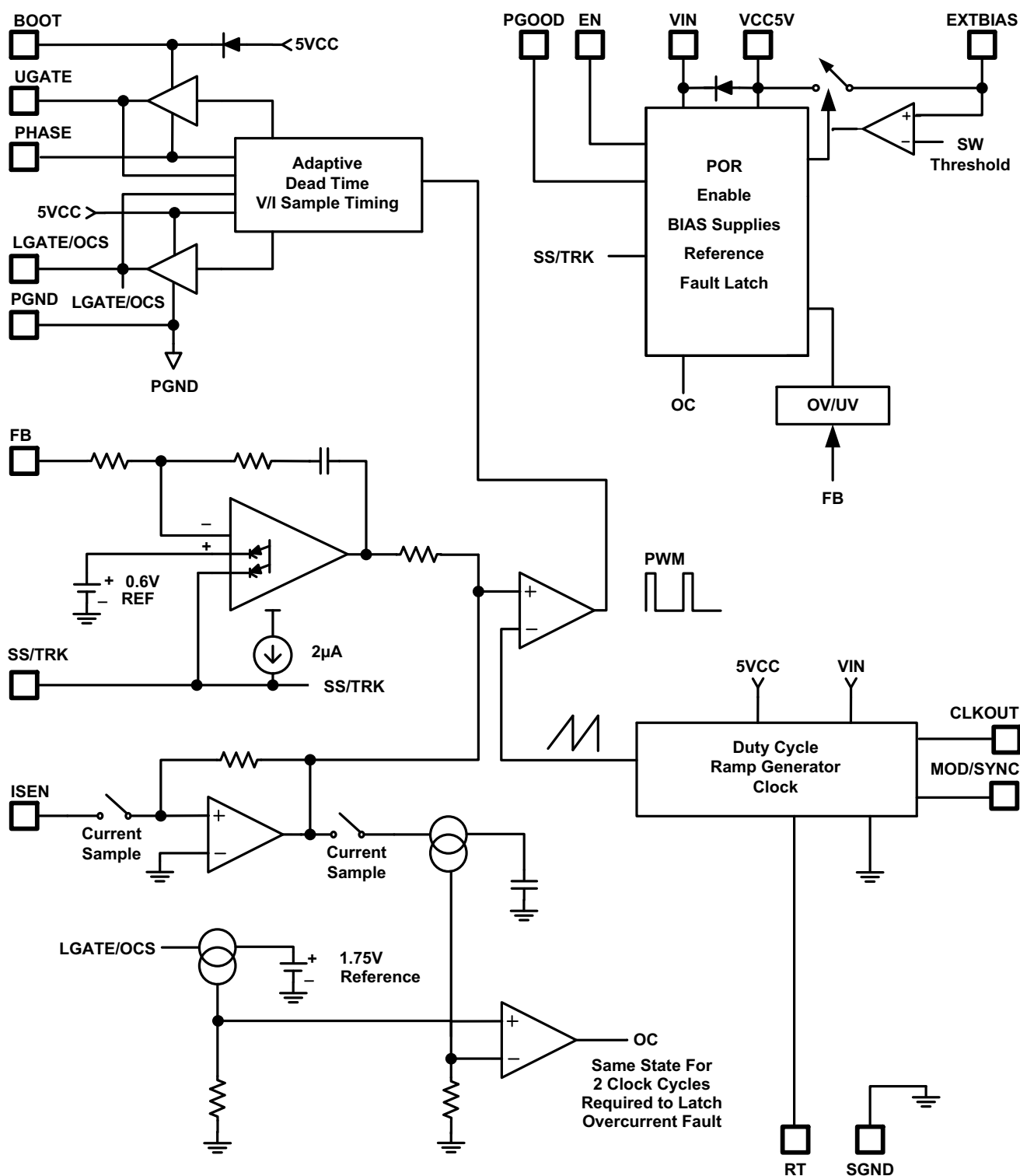
Figure 3. Block Diagram
