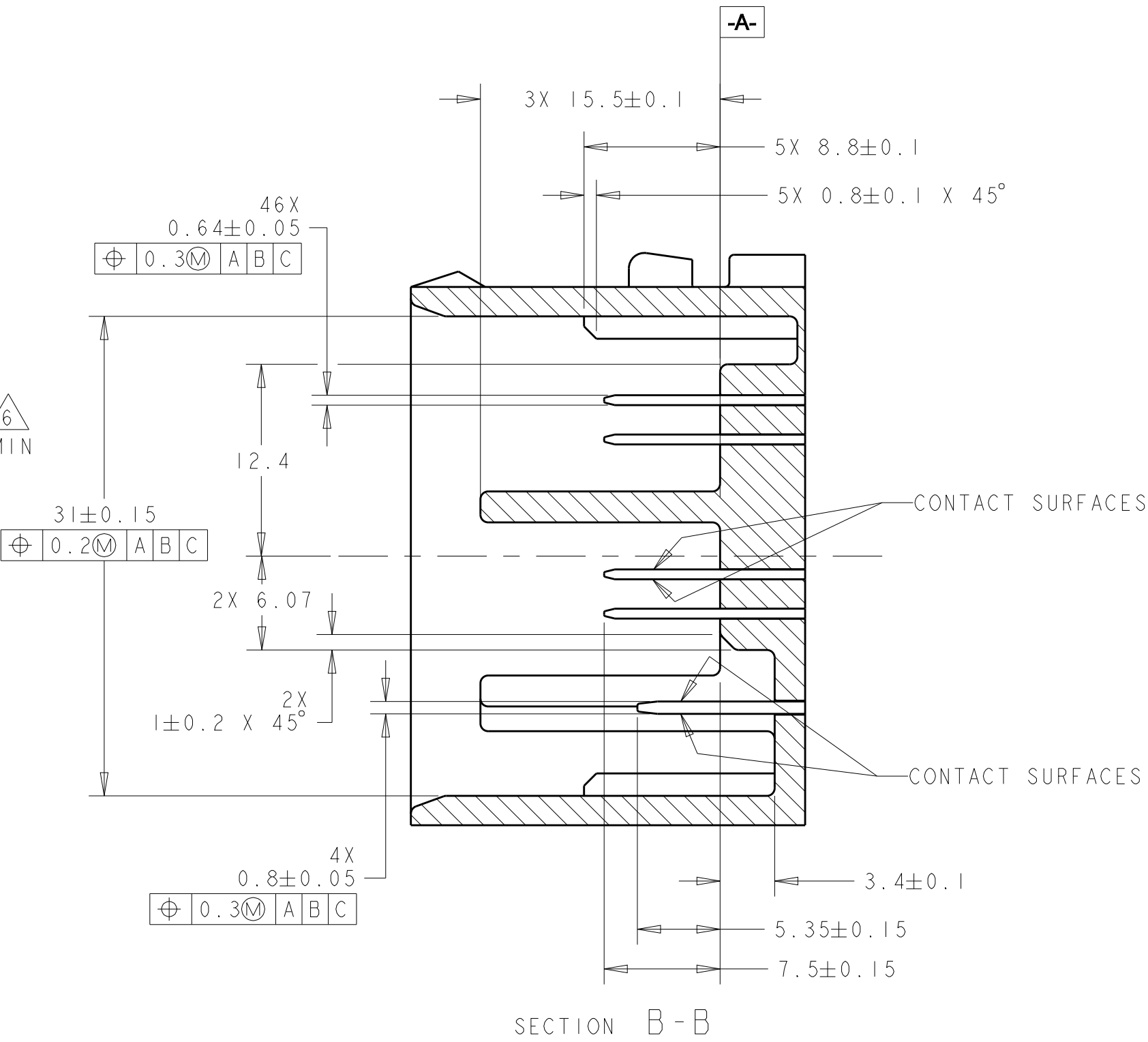
SECTION B-B
