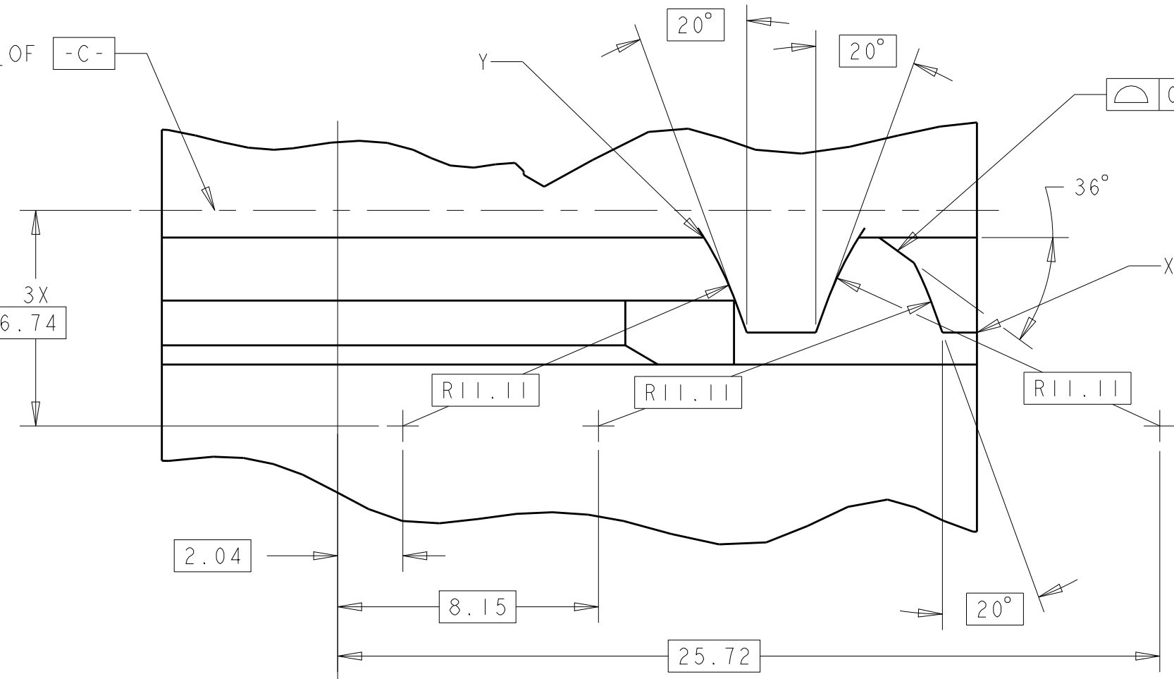
DETAIL G SCALE 6:1 2 PLC
