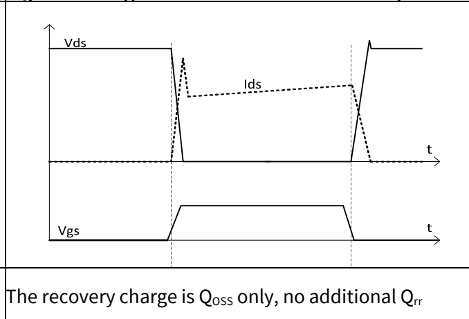
Figure 26 Typical Reverse Channel Recovery
