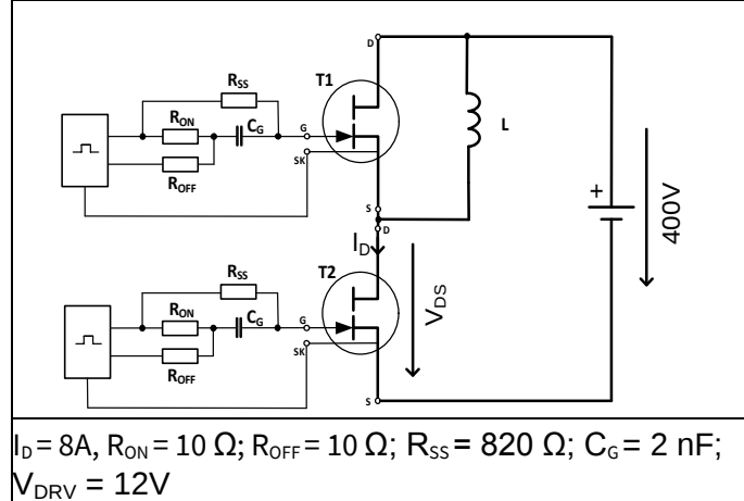
Figure 23 Switching times with inductive load
