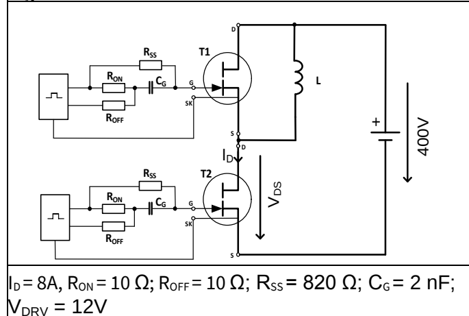
Figure 25 Reverse Channel Characteristics Test
