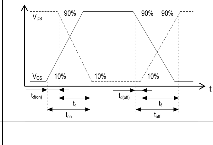
Figure 24 Switching times waveform
