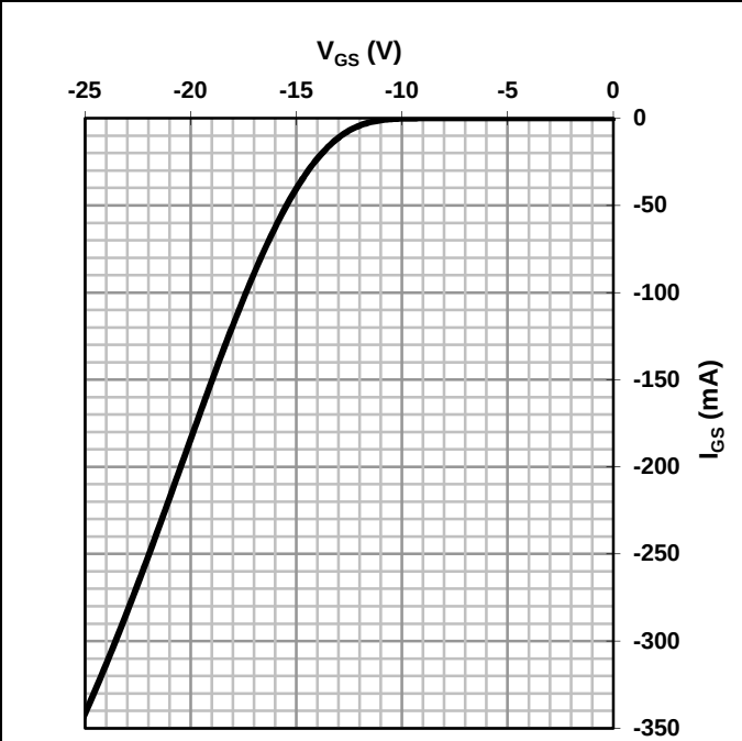
Figure 12 Typ. gate characteristics reverse
