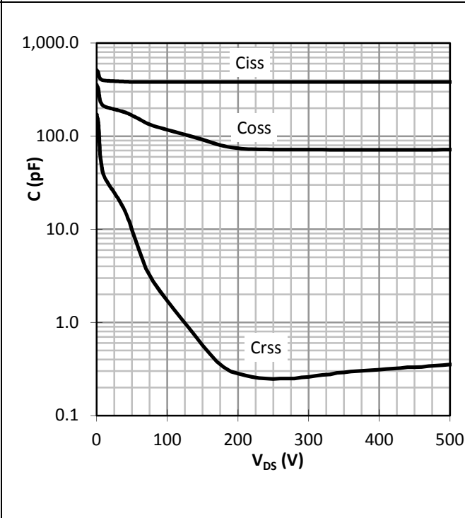
Figure 20 Typ. capacitances
