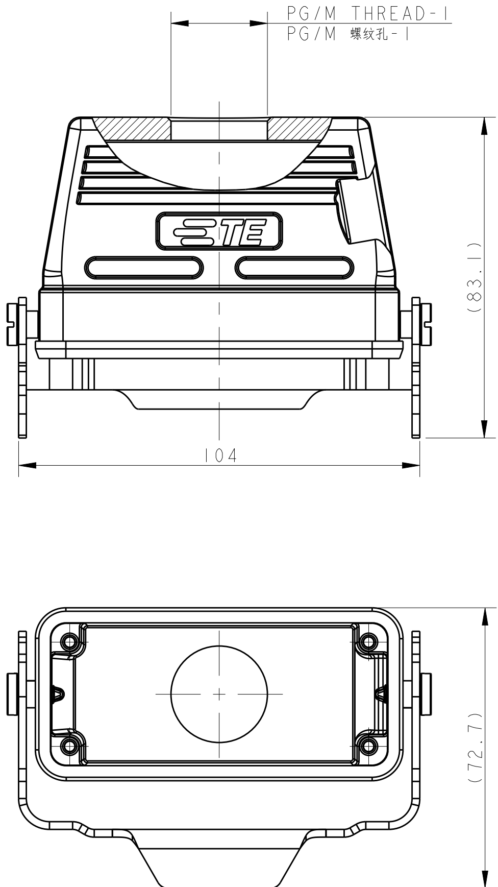
TYPE 4: LOW CONSTRUCTION + METAL SINGLE LOCKING OTHER SPEC REFER TO TYPE 1 类型4: 低结构壳体+彩钢单扣, 其他规格参照类型1
