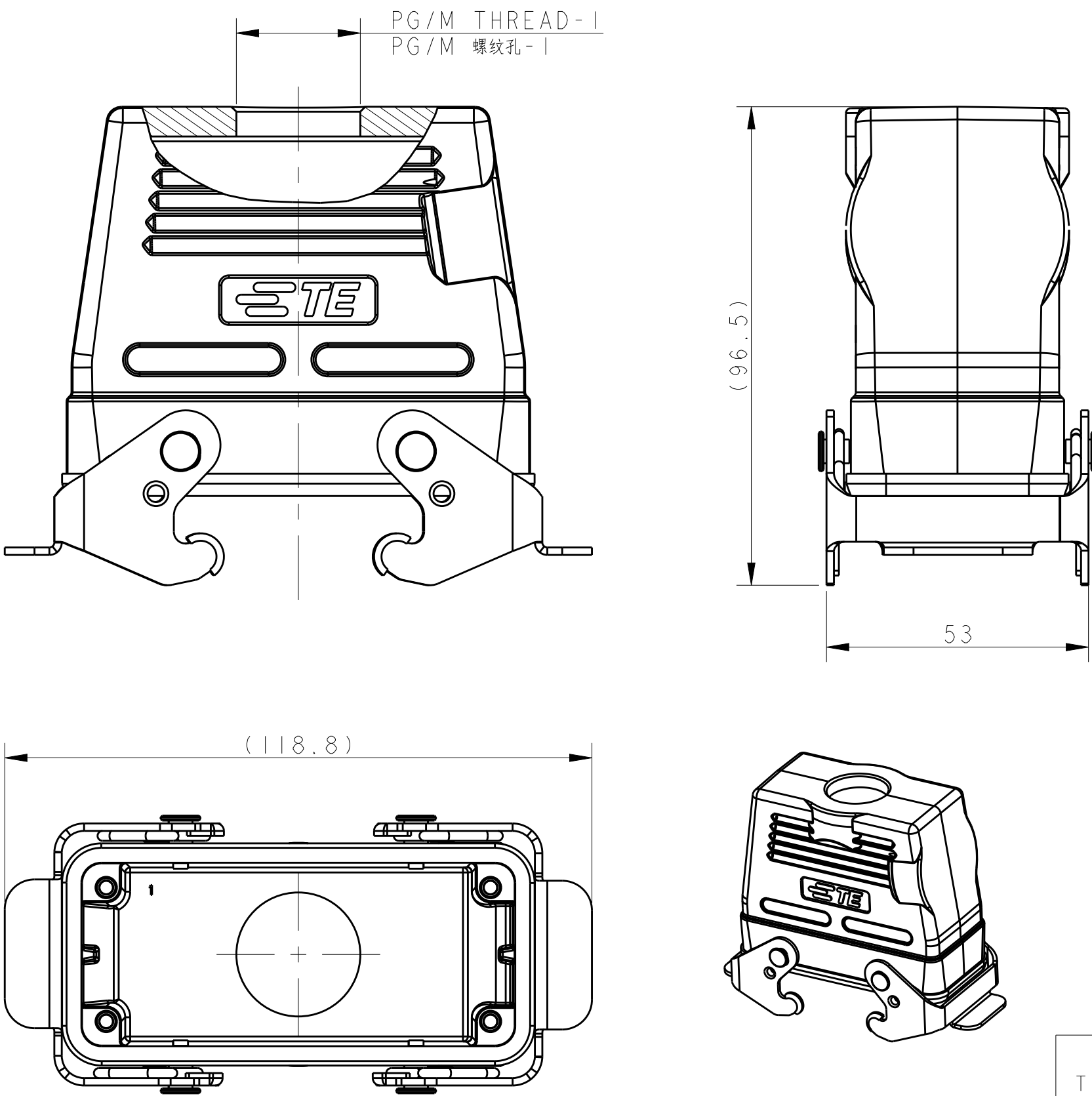
TYPE 6: HIGH CONSTRUCTION + METAL DOUBLE LOCKING
