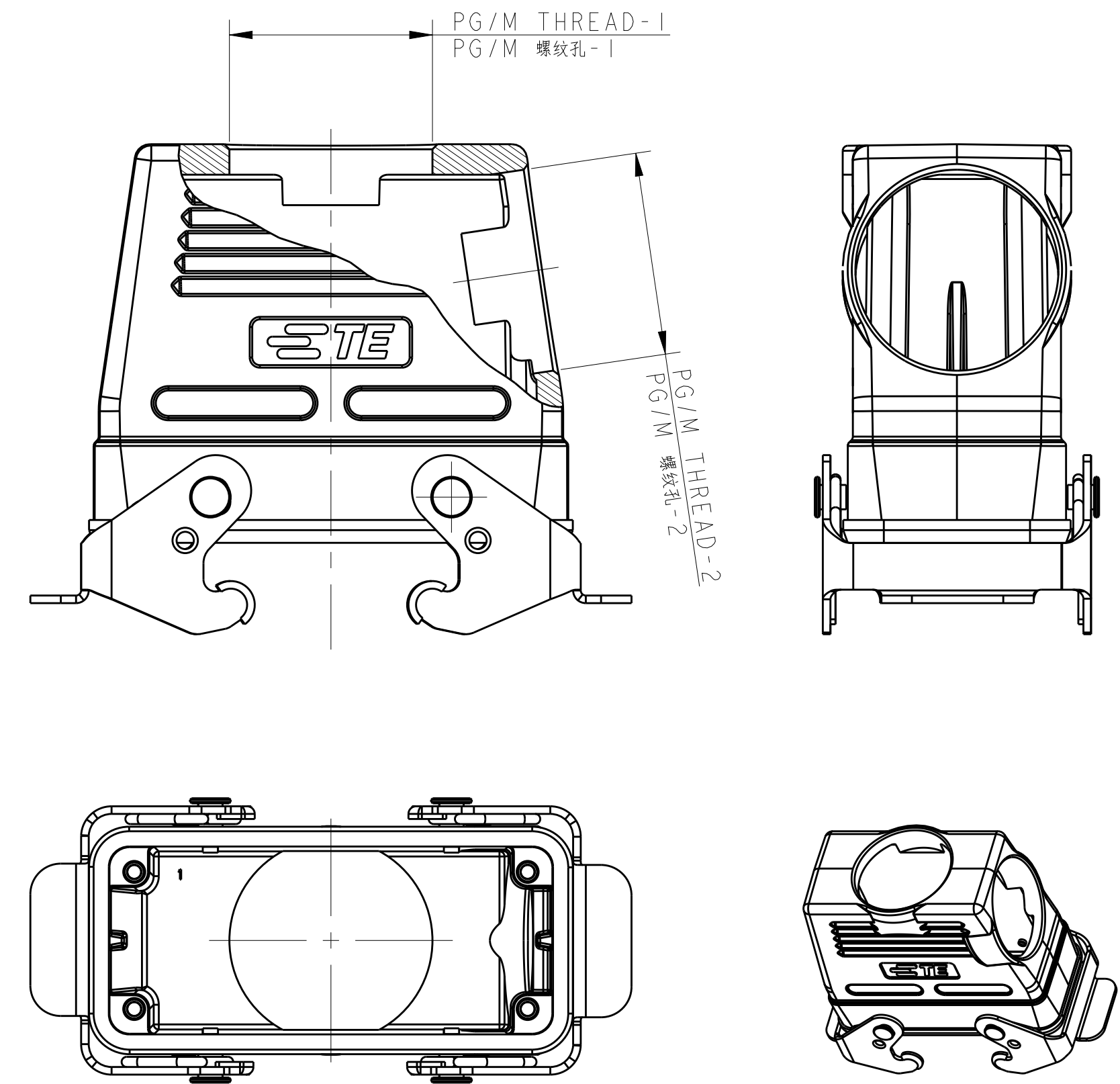
TYPE 8: HIGH CONSTRUCTION + METAL DOUBLE LOCKING
