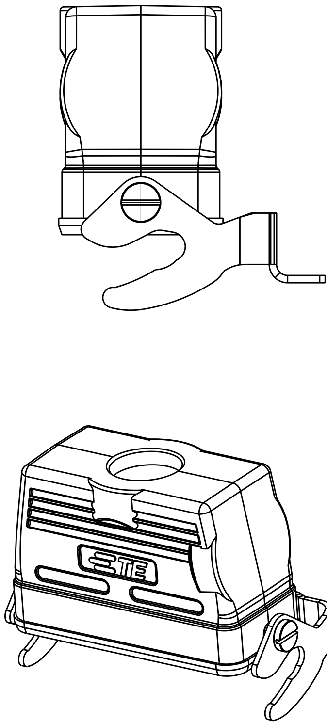
TYPE 4: LOW CONSTRUCTION + METAL SINGLE LOCKING OTHER SPEC REFER TO TYPE 1 类型4: 低结构壳体+彩钢单扣, 其他规格参照类型1
