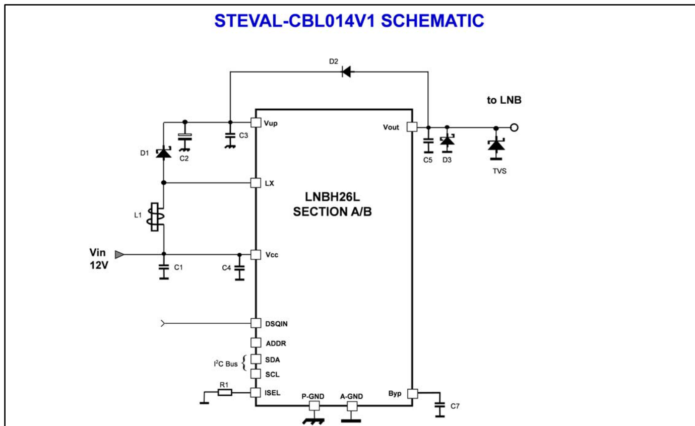
Figure 1: STEVAL-CBL014V1 schematic
