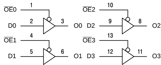
Figure 2. Logic Diagram
