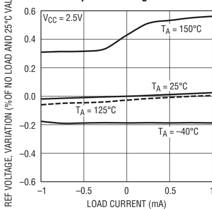
REF Output Load Regulation
