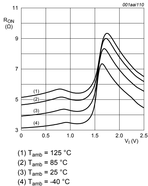
Fig. 10. ON resistance as a function of input voltage; V_{CC} = 2.5 V; I_{SW} = 24 mA
