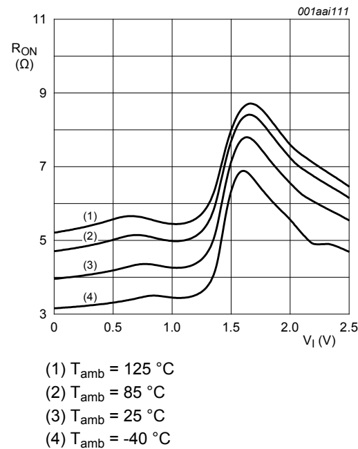
Fig. 11. ON resistance as a function of input voltage; V_{CC} = 2.5 V; I_{SW} = 64 mA
