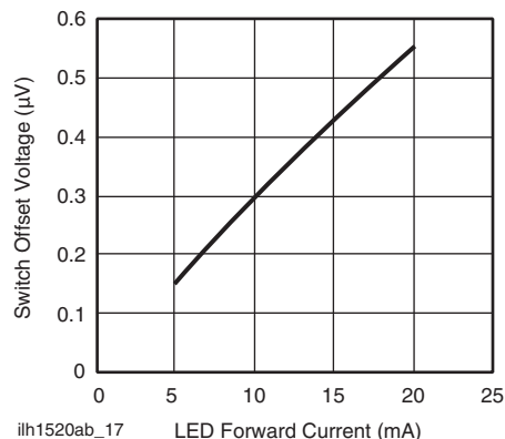
Fig. 18 - Switch Offset Voltage vs. LED Current
