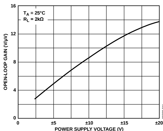
Figure 11. Open-Loop Gain vs. Power Supply Voltage
