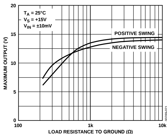
Figure 21. Maximum Output Voltage vs. Load Resistance
