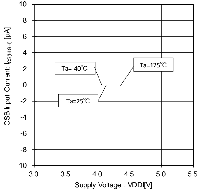
Figure 82. CSB Input Current- Voltage Characteristic (CSB=VDDI)
