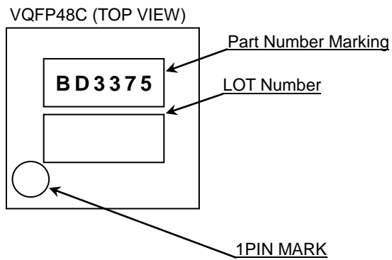
Figure 125. Marking Diagrams
