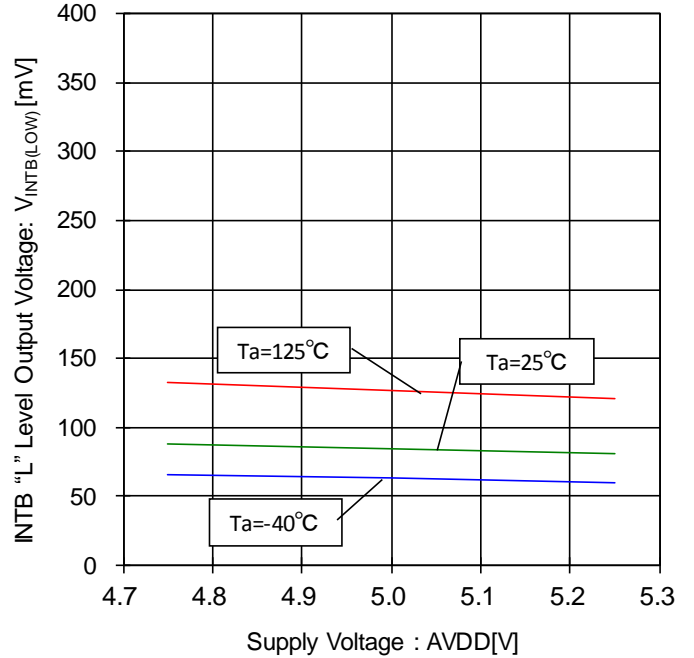
Figure 104. INTB "L" Level Output Voltage- Voltage Characteristic ( I_{SINK}=1.0\text{mA} )
