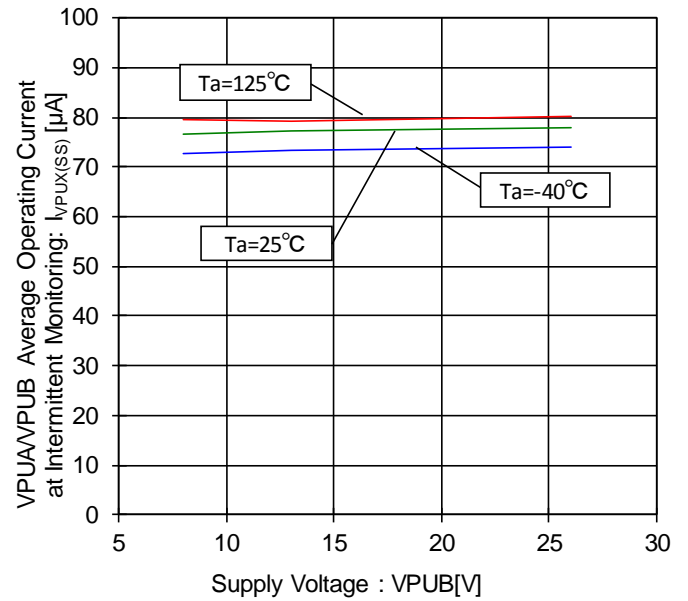
Figure 26. VPUA/VPUB Average Operating Current at Intermittent Monitoring - Voltage Characteristic (Monitoring Period: 50ms, Strobe Time: 125 \mu s , Source/Sink Current Setting: 1mA)
