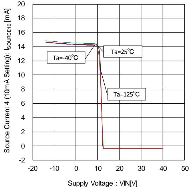
Figure 58. Source Current 4- Voltage Characteristic (10mA Setting)
