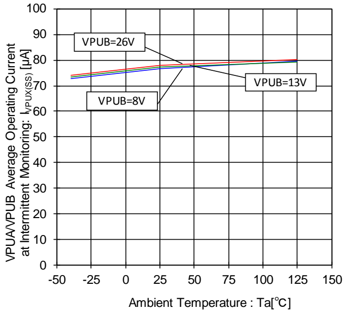
Figure 25. VPUA/VPUB Average Operating Current at Intermittent Monitoring - Temperature Characteristic (Monitoring Period: 50ms, Strobe Time: 125 \mu s , Source/Sink Current Setting: 1mA)
