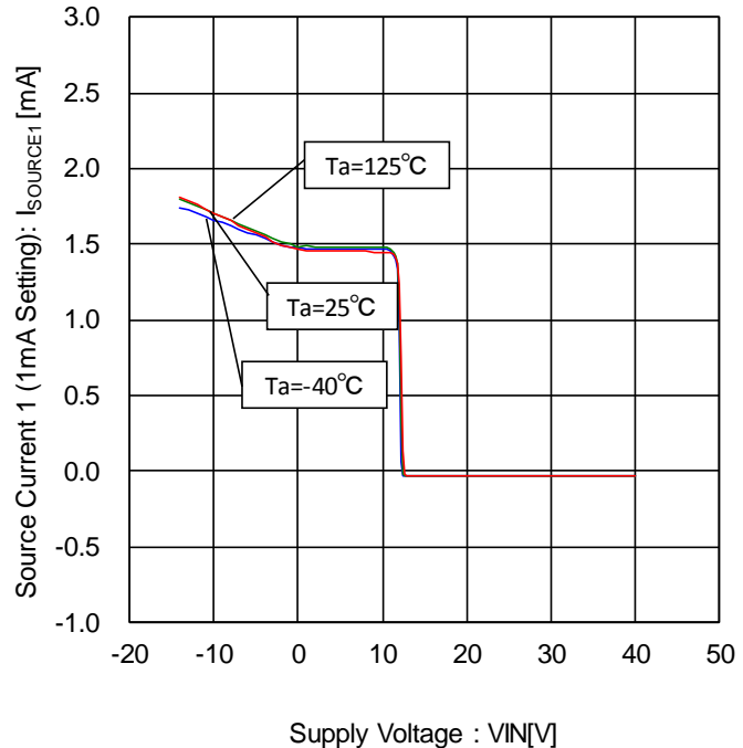
Figure 34. Source Current 1- Voltage Characteristic (1mA Setting)
