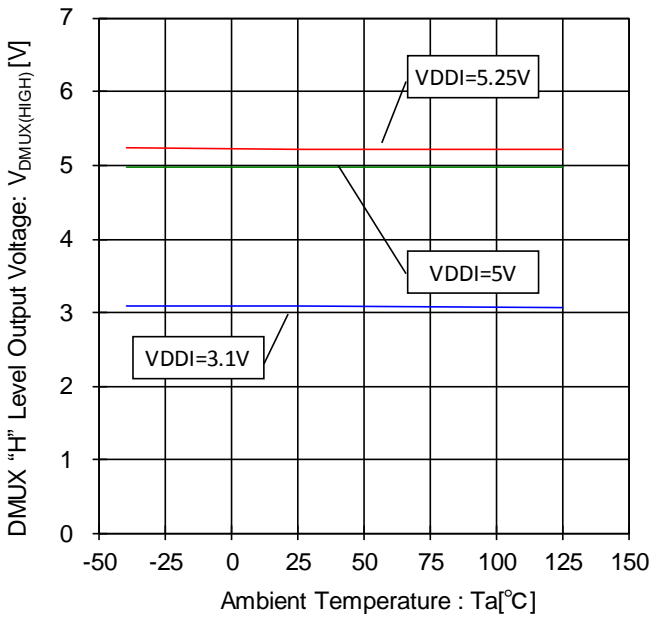
Figure 95. DMUX "H" Level Output Voltage- Temperature Characteristic ( I_{SOURCE}=200\mu A )
