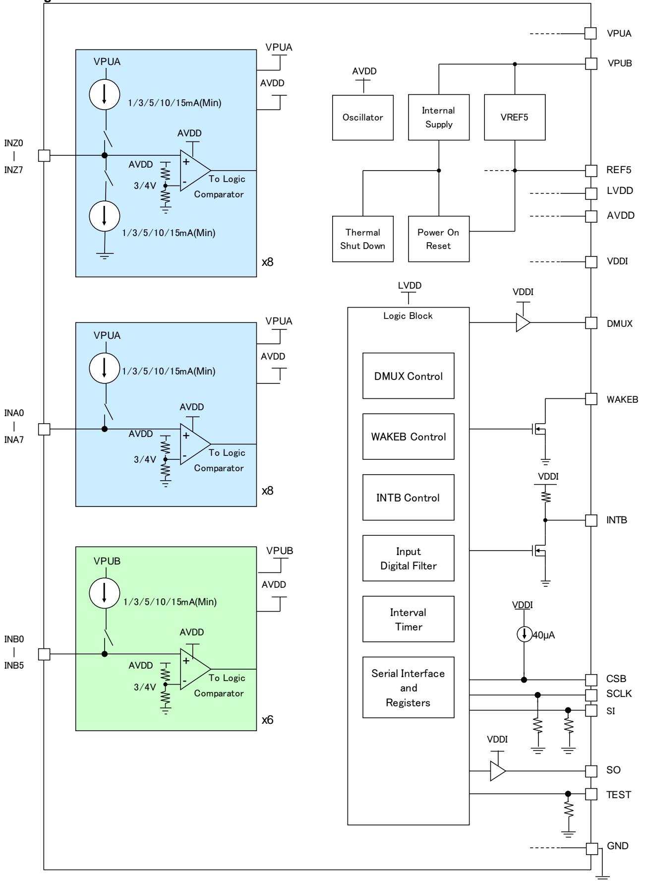
Figure 3. Block Diagram
