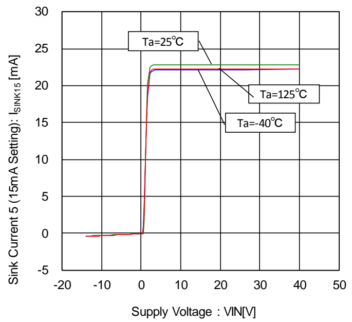
Figure 70. Sink Current 5- Voltage Characteristic (15mA Setting)
