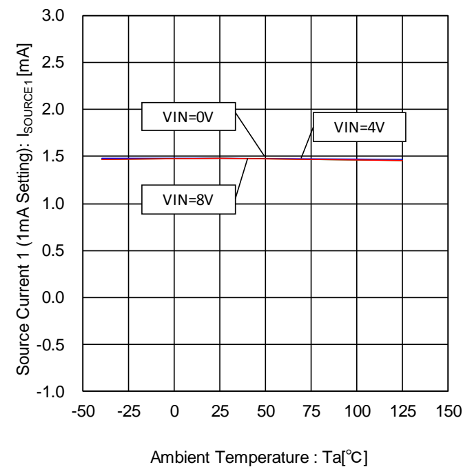
Figure 33. Source Current 1- Temperature Characteristic (1mA Setting)
