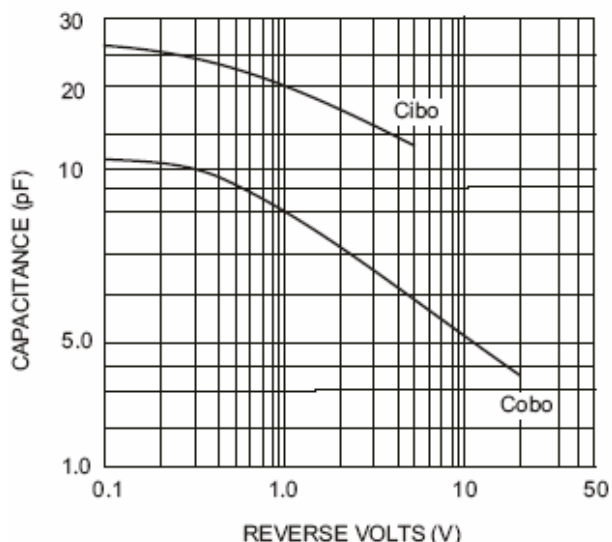
Fig. 3 Typical Capacitance
