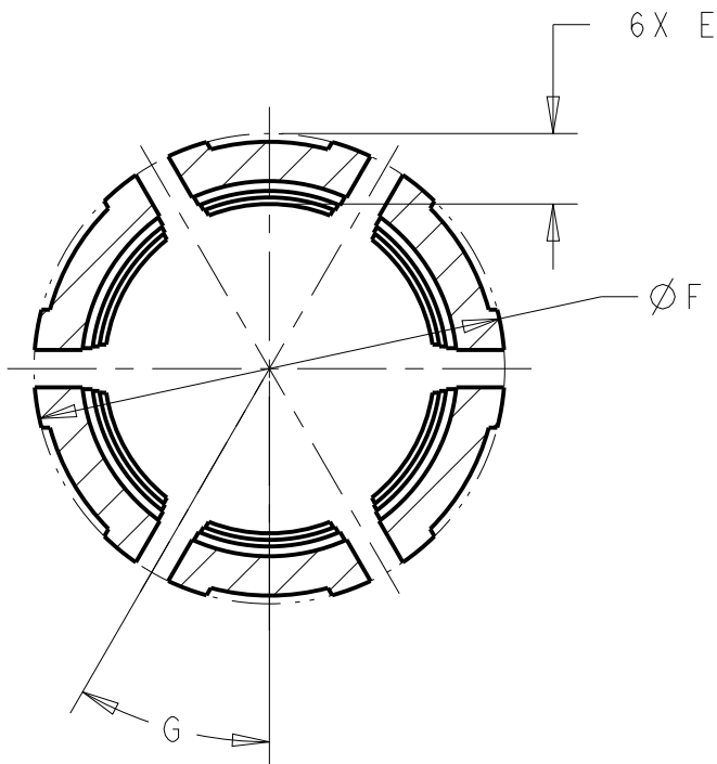
SECTION B-B
