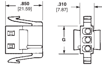
Socket Housing (Plug)
