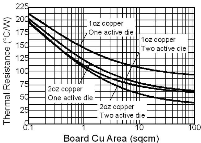
Thermal Resistance v Board Area
