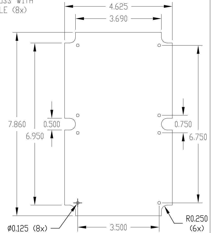
SUGGESTED PC BOARD LAYOUT
