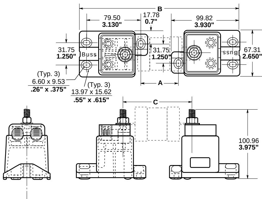
Dimensional Data \frac{\text{mm} (\pm .25)}{\text{Inches} (\pm .01)}
