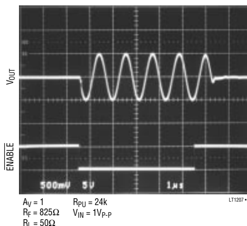
Figure 3. Shutdown Operation
