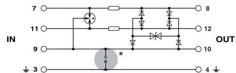
Circuit diagram
