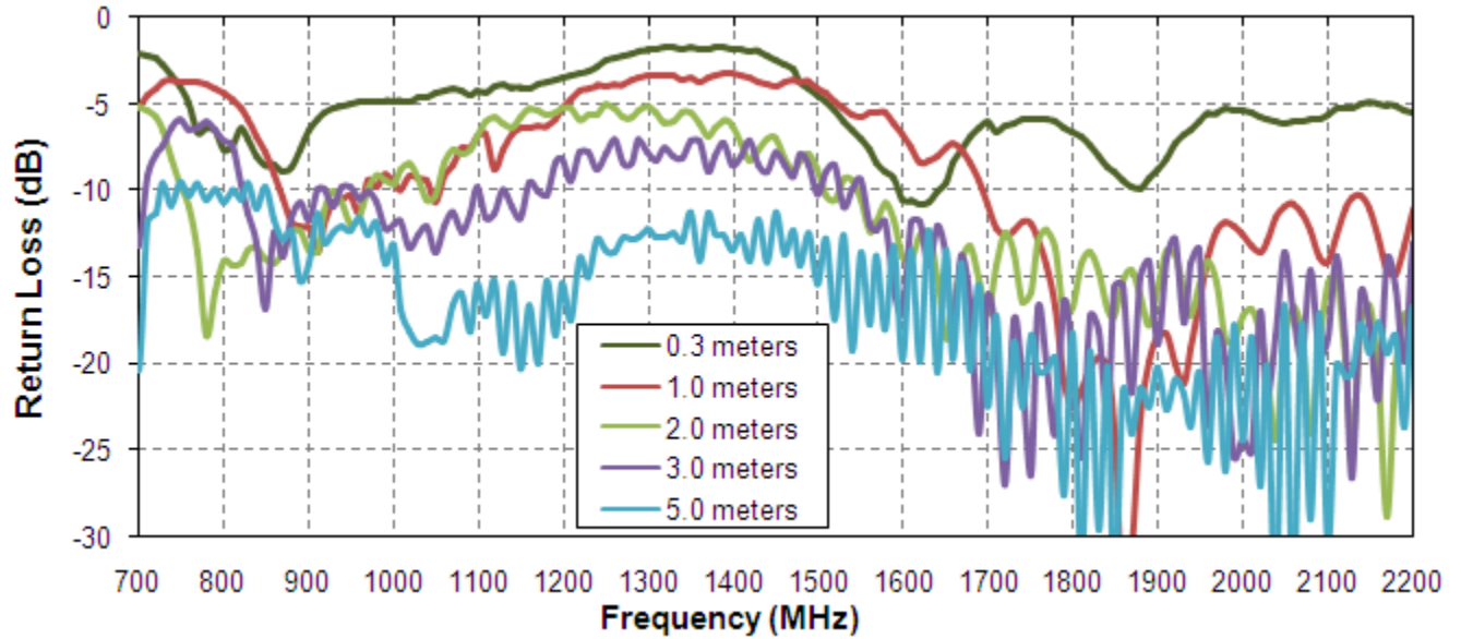
Figure 4. Return Loss of the MA104 antenna on 60*60cm metal plate
