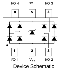
Device Schematic
