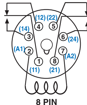
8 PIN
