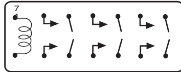
219FXXP 6P-NO
