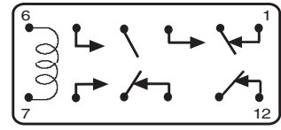
219ABAP DPDT+1NO & 1NC
