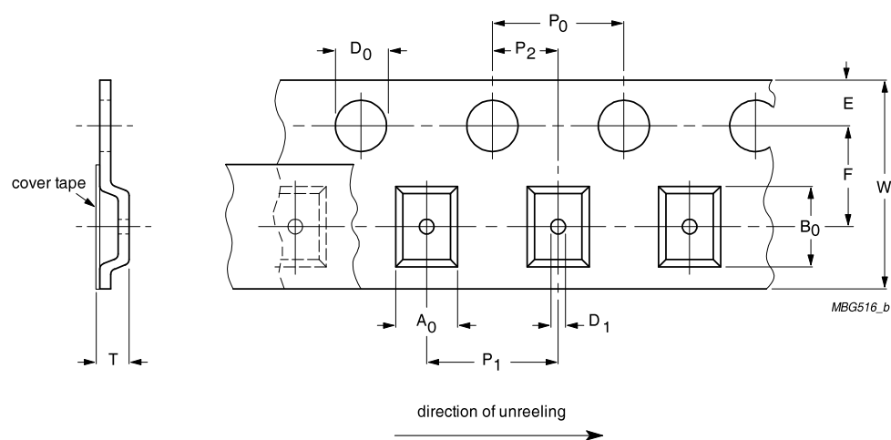
Fig. 6 Embossed Tape
