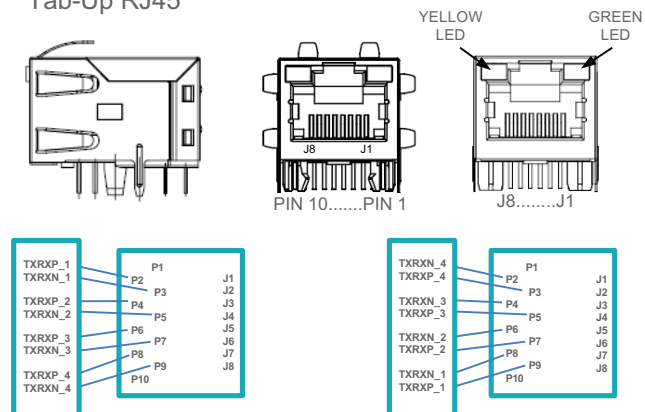
Clockwise Orientated PHY JXD1-0025NL / JXD1-0026NL
