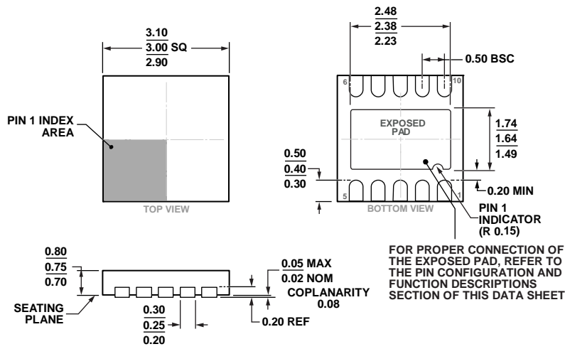
Figure 50. 10-Lead Frame Chip Scale Package [LF CSP] (CP-10-9) 3 mm × 3mm Body, Very Thin, Dual Lead Dimensions shown in millimeters
