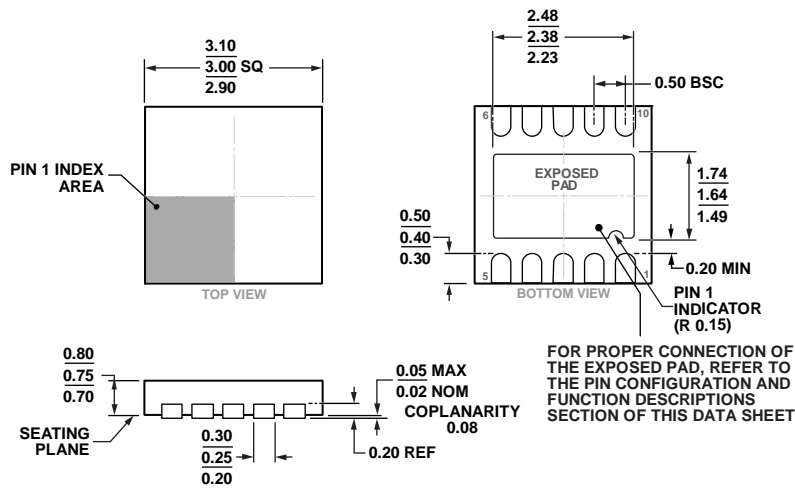
Figure 50. 10-Lead Frame Chip Scale Package [LF CSP] (CP-10-9)
