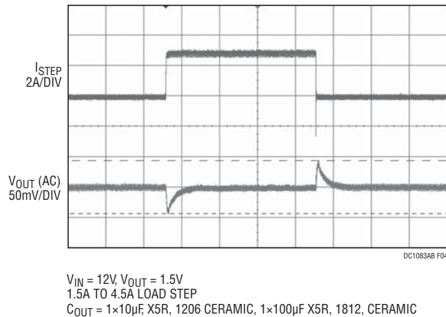
Figure 4. Measured Load Transient Response (3A Step)
