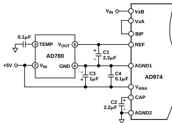
Figure 15. External Reference to AD974 Configured for \pm 10 V Input Range
