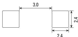
recommended Pad Layout (mm)
