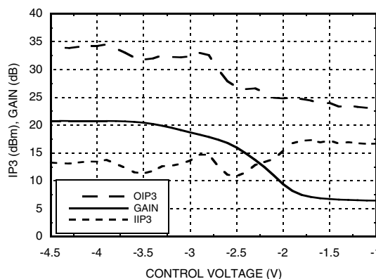
IP3 and Gain @ 22 GHz Pin = -20 dBm
